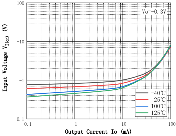
Fig.1 - ON Characteristics
