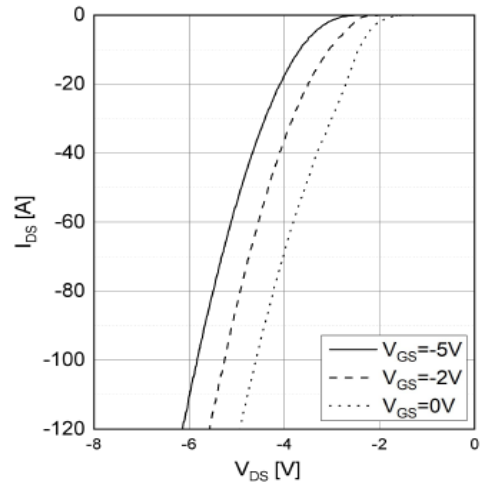
Figure 8. Reverse Output Characteristics at Tj = 25°C
