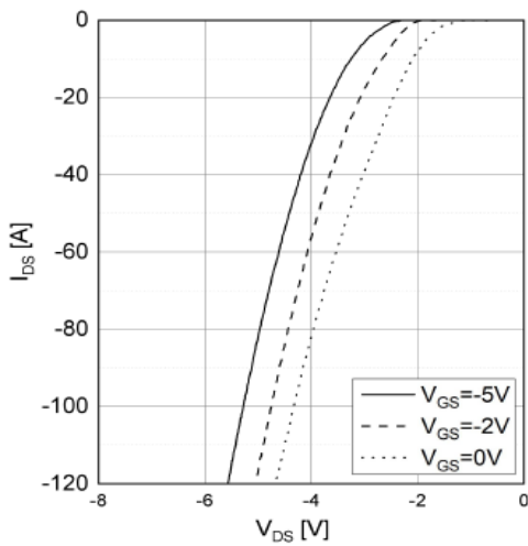
Figure 9. Reverse Output Characteristics at Tj = 175°C
